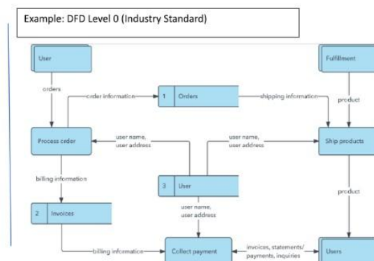
Figure 1: Simplified system flow and Level 0 Industry Standard DFD for BookStore application.
